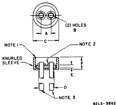
Figure 7: Typical Coolant Connection (Except Anode)
