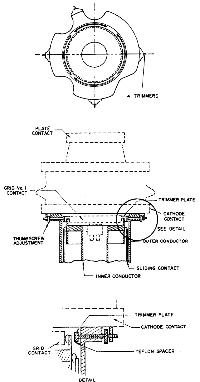
Figure 2: Input Cavity Section
