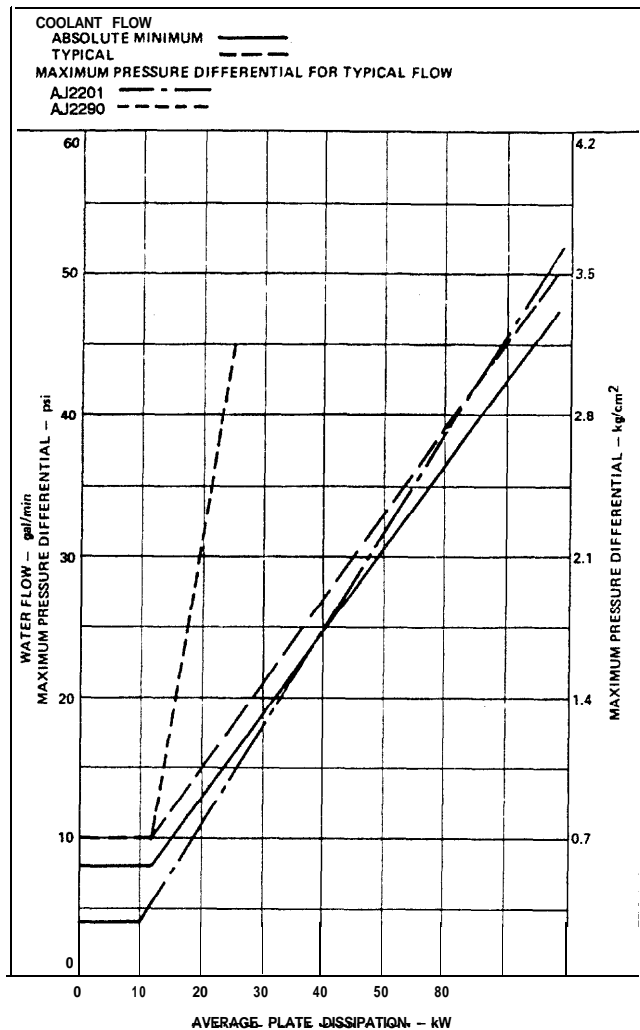
Figure 1: Plate Coolant Specifications
